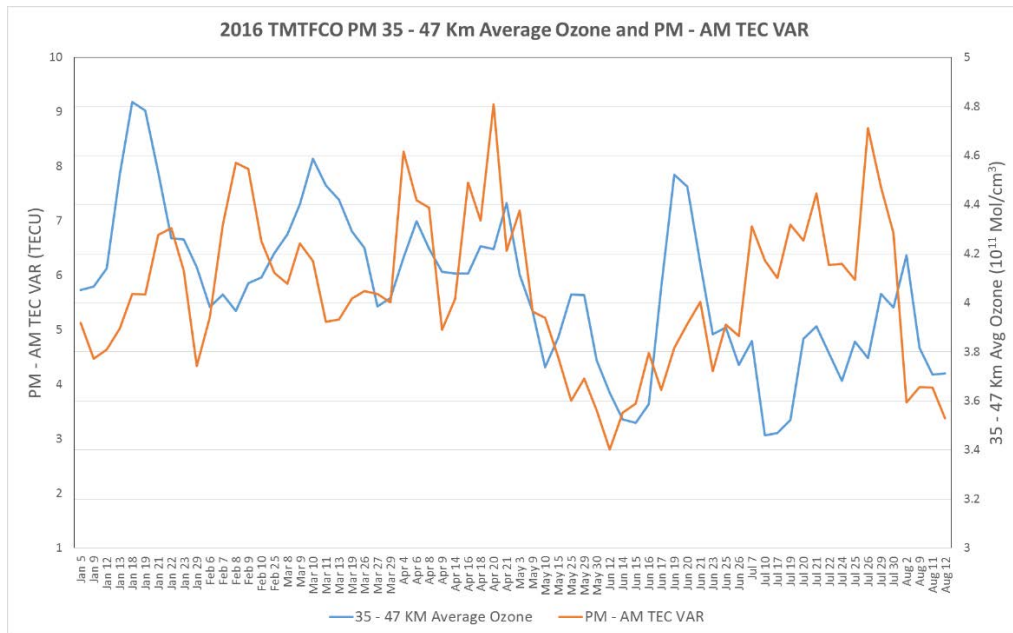
Figure 5: TMTFCO PM Time Series
