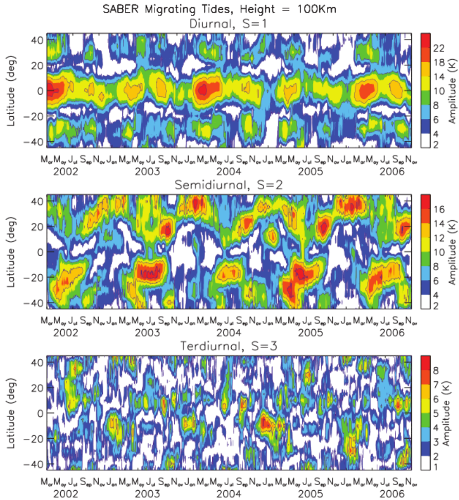
Figure 1: Migrating Tides Thermal Amplitudes (Forbes, 2008) Diurnal, semidiurnal, and terdiurnal thermal amplitudes at 100 Km for latitudes between 45S and 45N. Based on SABER measurements conducted from Mar 2002 through November 2006.
