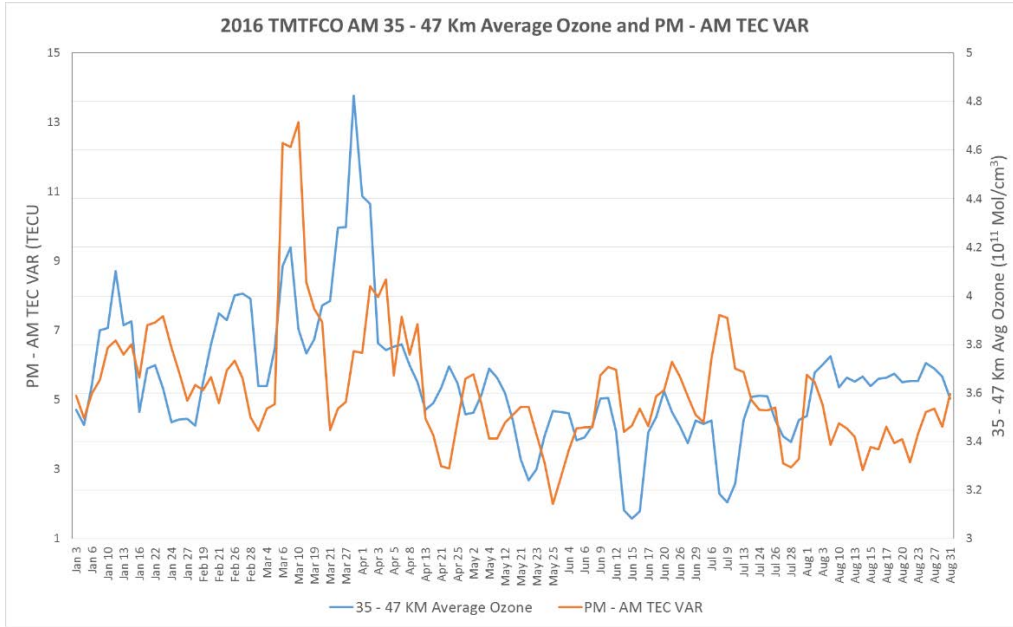
Figure 4: TMTFCO AM Time Series
